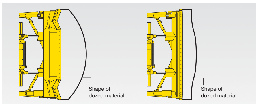
Up to 15% higher production with the improved Sigadozer® blade (left), compared to conventional Semi-U blade (right).
